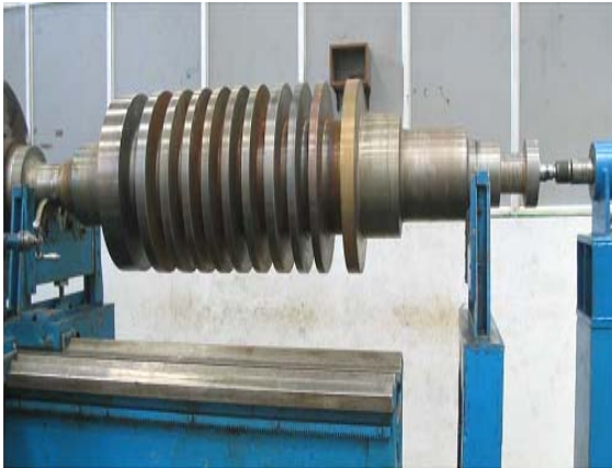
Rotor Shaft Forging in Proof machined condition after stress relieving
